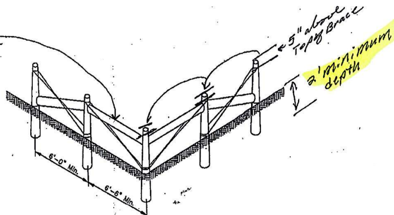
5-POST CORNER PANEL (TYPE I)
