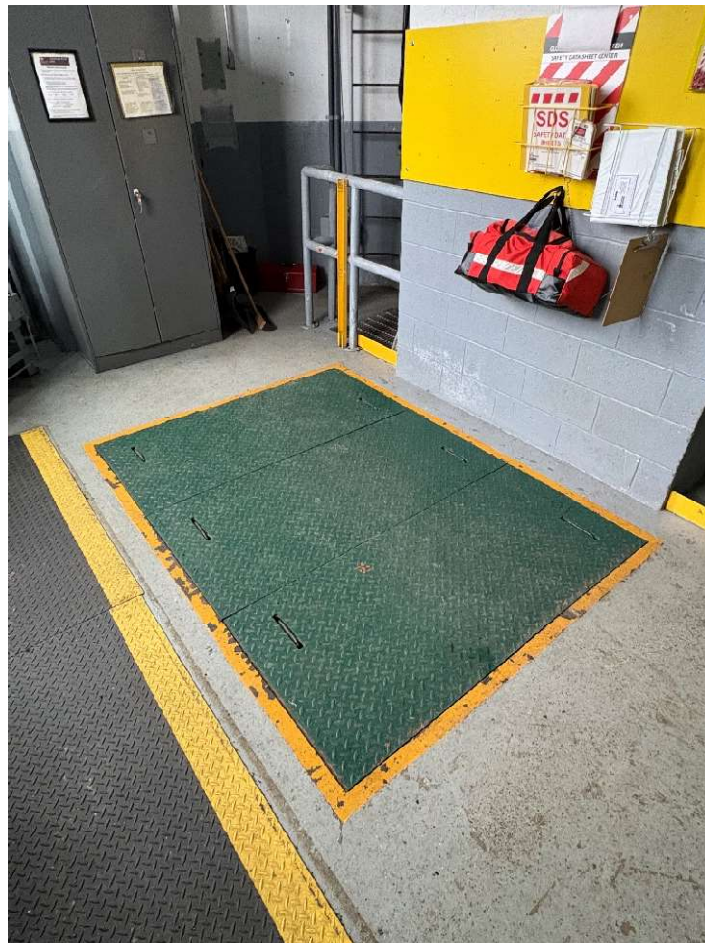
Colebrook River Lake Main Level Hatchway, Approximately 5' x 7' with Panels Removed
