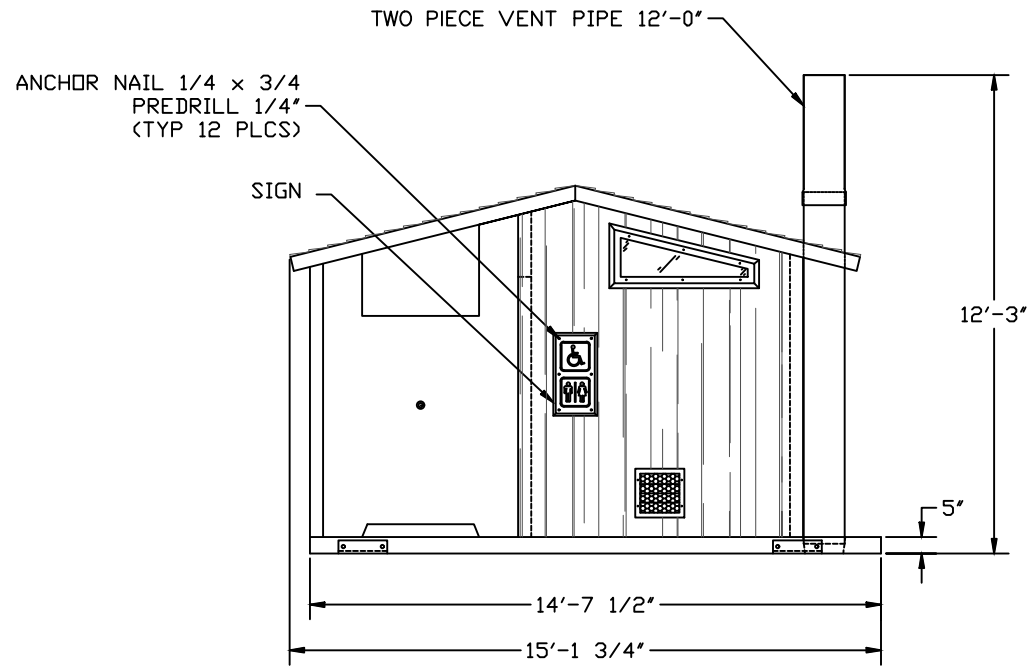
FRONT ELEVATION
