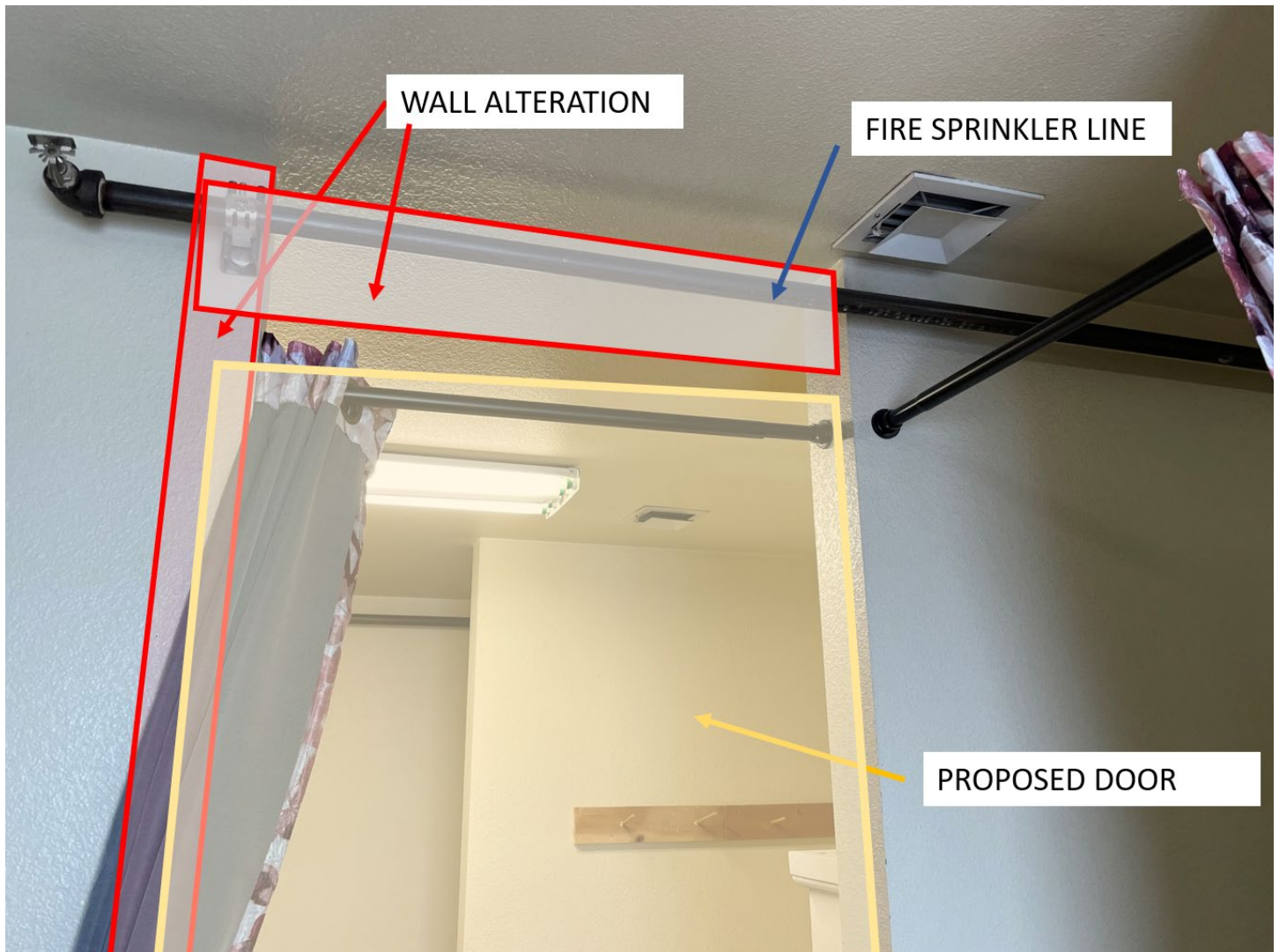
Proposed bathroom door.
