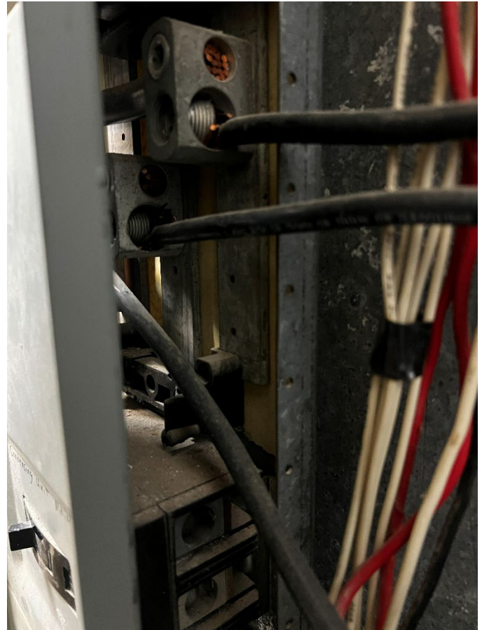
Figure 7: EXISTING ELECTRICAL, DIRECT CONNECTION TO PANEL BUS BAR.
