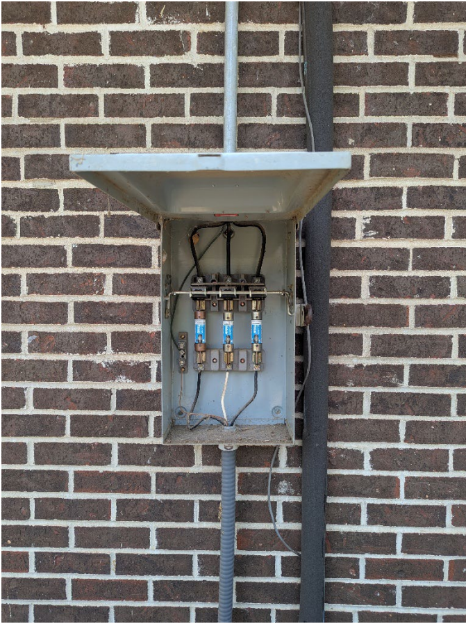
Figure 9: HEAT PUMP DISCONNECT.
